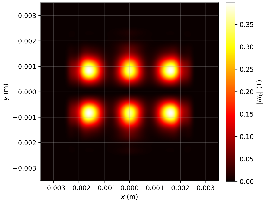
Intensity profile I(x, y, z = 3.503)/I_0 , \text{Pin}=3.0\text{Pcr} , artificial time
